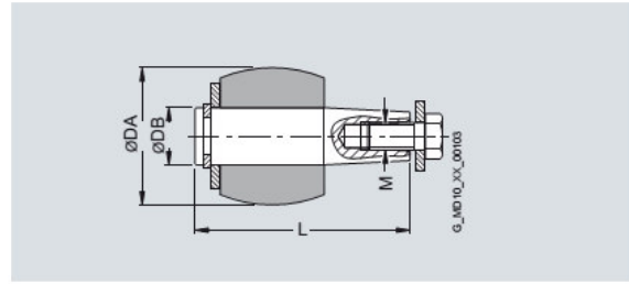
Sizes 710 ... 2000
