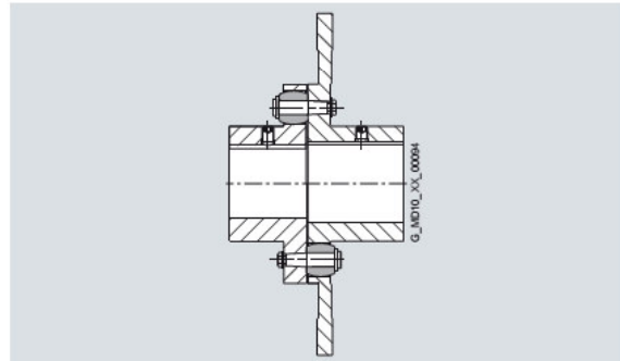
Types RWB/RBS with brake disk
