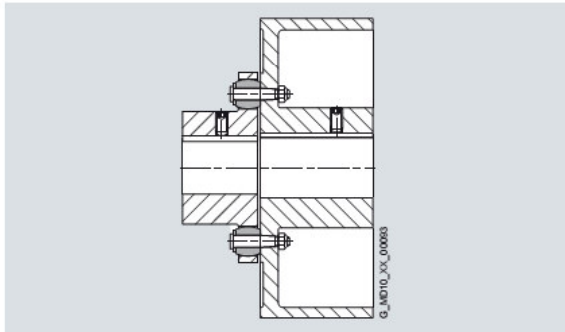
Types RWB/RBS with brake drum
